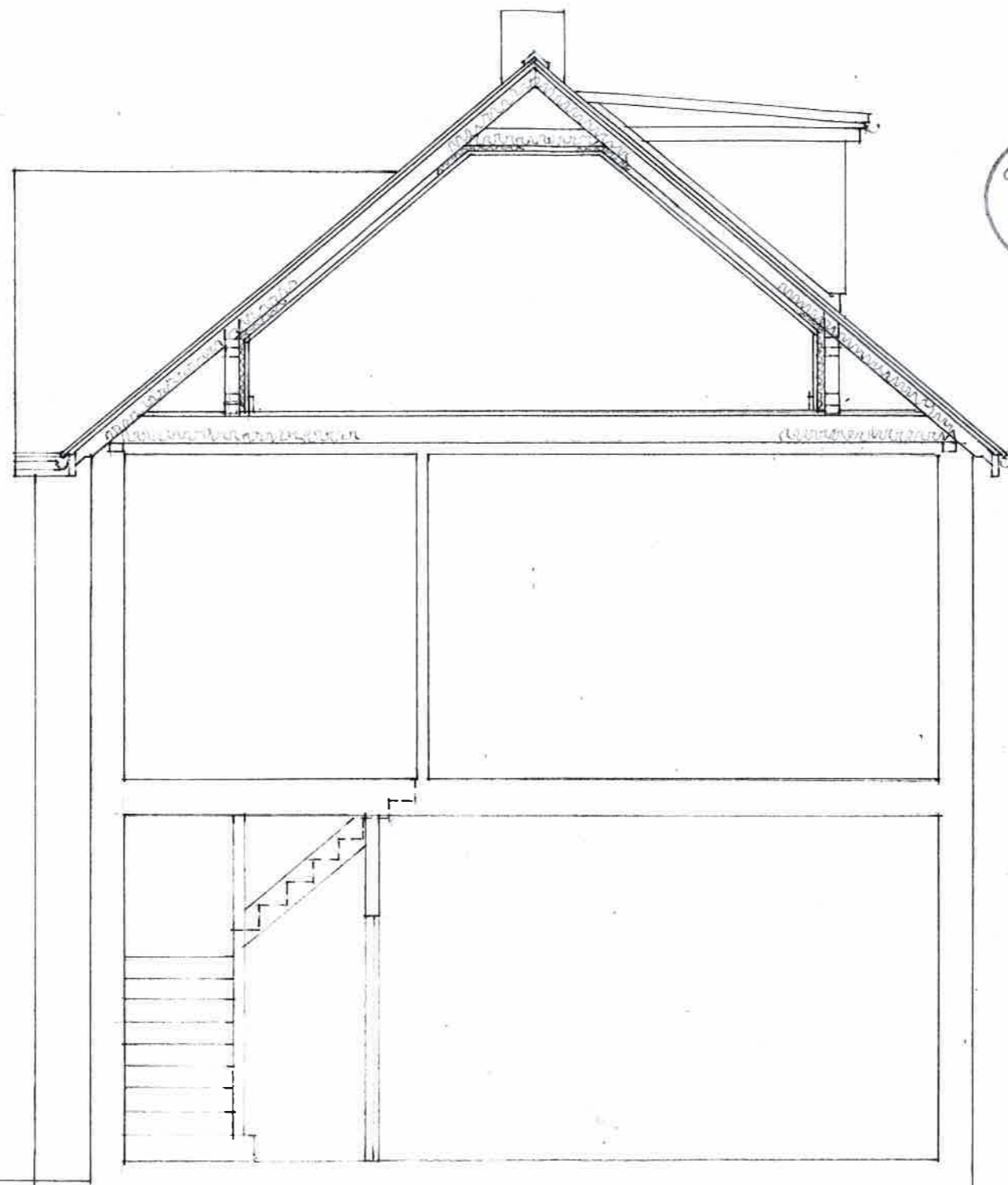
SECTION D-D AND NORTH ELEVATION TO DORMER
